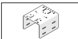
Shifter Plate
