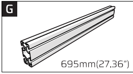
Aluminum Profile AP-8040-695 X2
