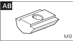
Ball Bearing Nut N5-M8 X86
