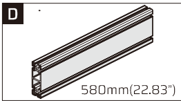
Aluminum Profile AP-40120-580 X1
